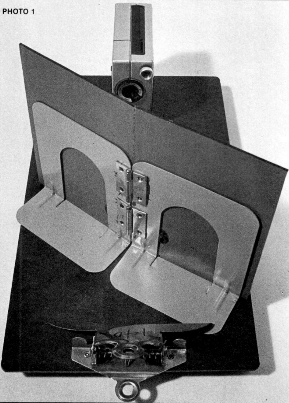
3-D camera system consists of two mirrors, a pair of bookends and a clipboard. Bookend closest to the camera should be glued firmly to the clipboard; the other should be left unglued so it can be repositioned when the clip is raised.
